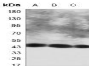
Western blot analysis of Cytokeratin 18 expression in HeLa (A), COS7 (B), 293T (C) whole cell lysates.
