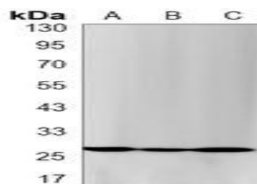
Western blot analysis of PCNA expression in mouse spleen (A), K562 (B), C6 (C) whole cell lysates.
