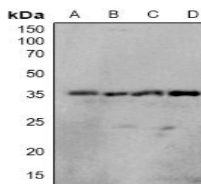
Western blot (WB) analysis of OTUB1 (Phospho-S187) polyclonal antibody at 1:500 dilution
