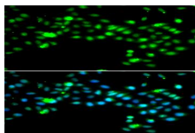
Immunofluorescence analysis of MCF7 cell using SRSF4 antibody.
