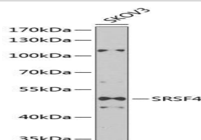
Western blot analysis of SRSF4 antibody.
